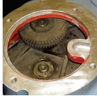
After: Actuator after overhaul and refurbishment by Weir Power & Industrial.
