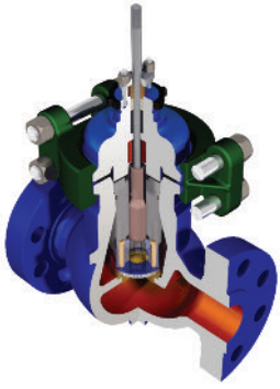
Weir's X-Stream™ severe service control valve.
