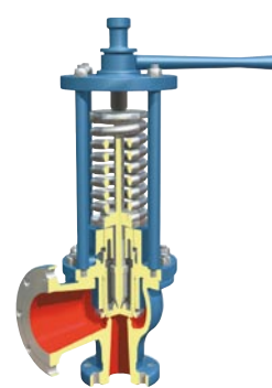
A7000 Series (Steam boiler) ISO 4126 (+3% overpr.) Semi nozzle Sizes : 2" - 6" Set P : upto 150 barg Temp : upto +565°C Mat : CS - AS - SS
