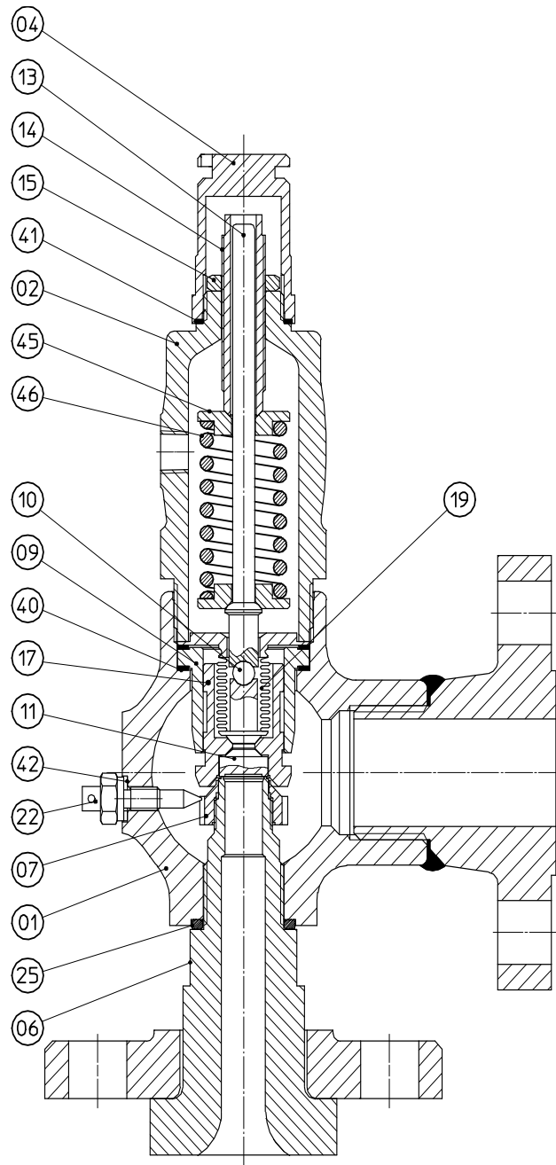
SOUPE EQUILIBREE BALANCED SAFETY VALVE
